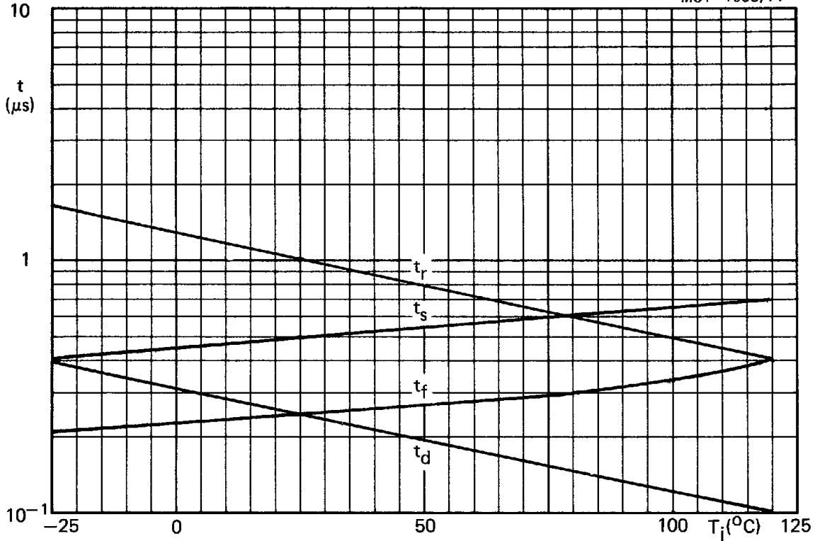
Fig.14 Switching times as a function of junction temperature; V_D \geq 250 V; I_T = 5 A; I_{GF} = 0.5 A; V_{GR} = 10 V; I_G = 0.2 A; L_G = 0.8 μH; maximum values.
